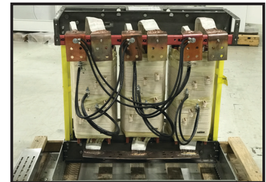
Dry Type Isolation Transformer
